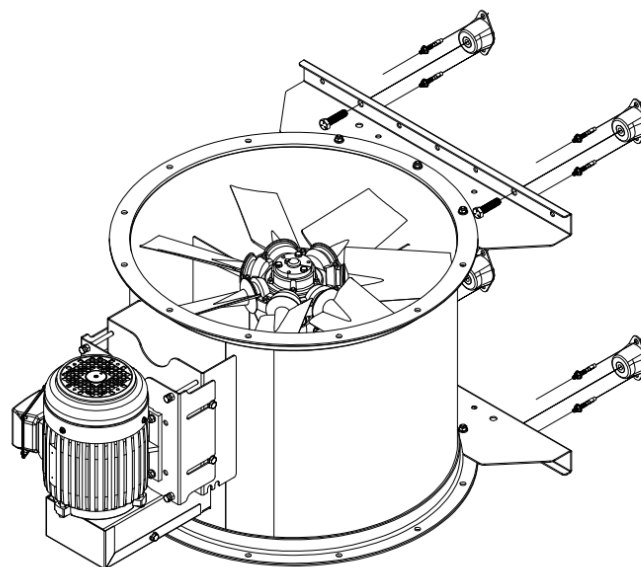
Figure 2 - Tube Axial Fan shown with Vibration Isolator Kit
