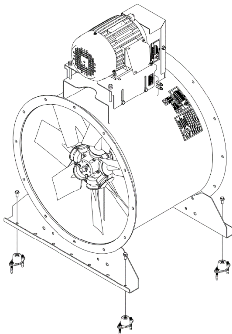
Figure 2 - Tube Axial Fan shown with Vibration Isolator Kit
