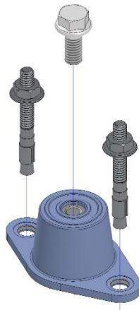
Figure 1 - Vibration Isolator with Fasteners
