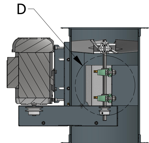
SECTION C-C SCALE 1/10
