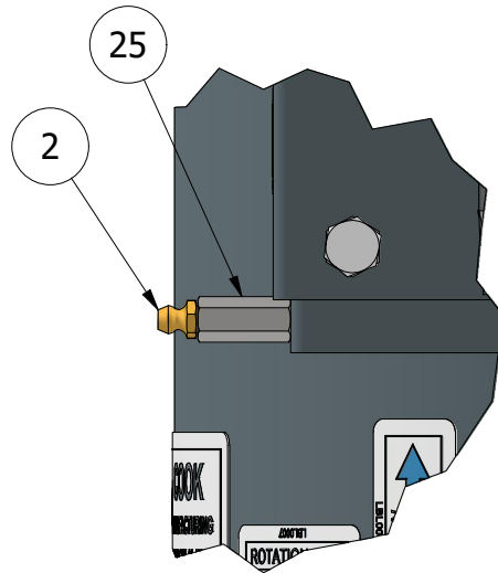
DETAIL E SCALE 1/2
