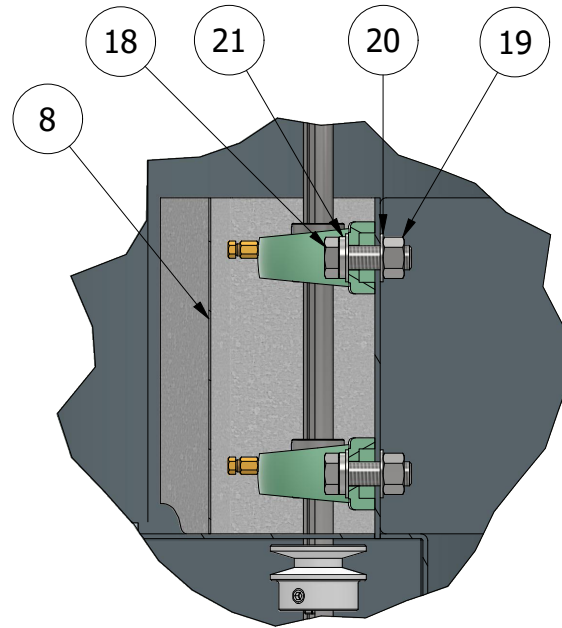
DETAIL D SCALE 1 / 4
