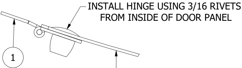
DETAIL B SCALE 1/1
