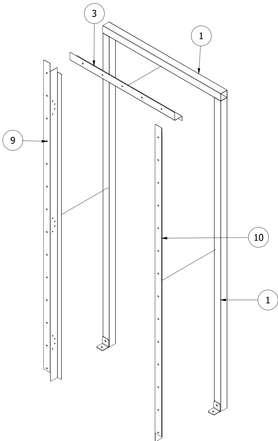
EXPLODED VIEW
