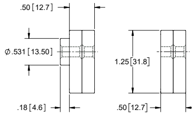
RIGHT SIDE VIEW WITH STUDS
